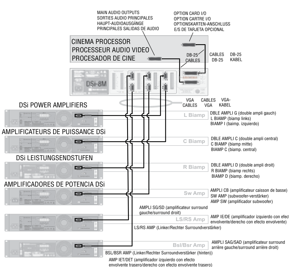
Figure 2.3 Wiring DSi Amplifiers to DSi-8M Monitor Panel with HD-15 Connectors
