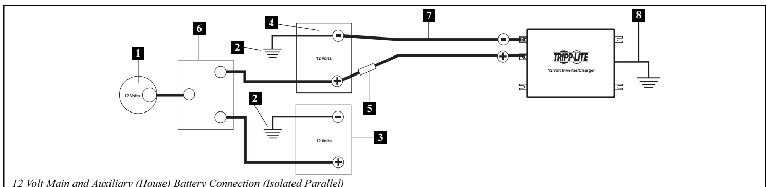
12 Volt Main and Auxiliary (House) Battery Connection (Isolated Parallel)
