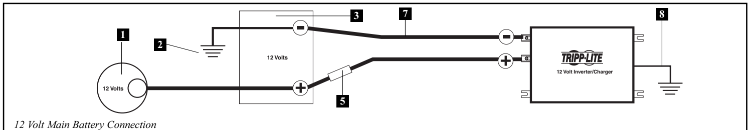
12 Volt Main Battery Connection
